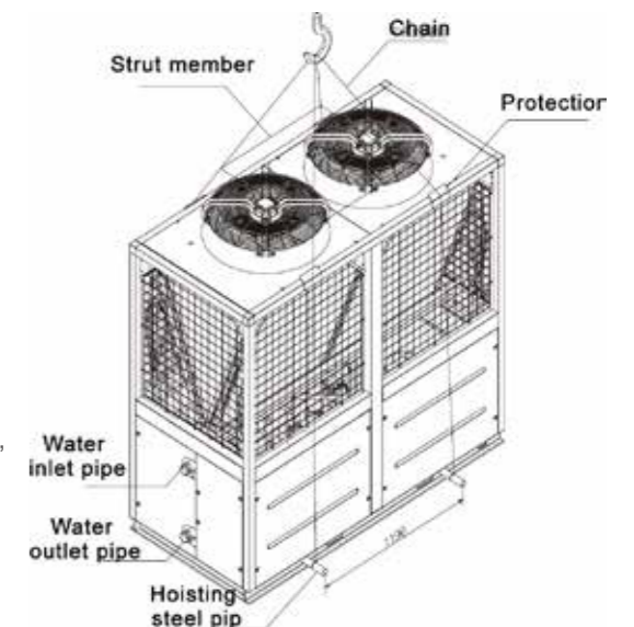
Example lifting schematic for TCA201
